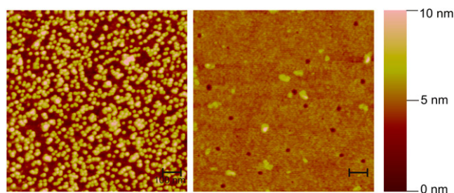
FIGURE 1 Imaging by AFM of glass coverslips coated with BSA alone (right panel) or with BSA and 5 nm colloidal gold (left panel). The images were recorded in tapping mode and represent the height range in false colors with maximal height of 10 nm (brightness scale on the right). Notice that gold particles appear slightly bigger than their actual size of 5 nm due to the resolution limits of the cantilever. Scale bar = 100 nm.
